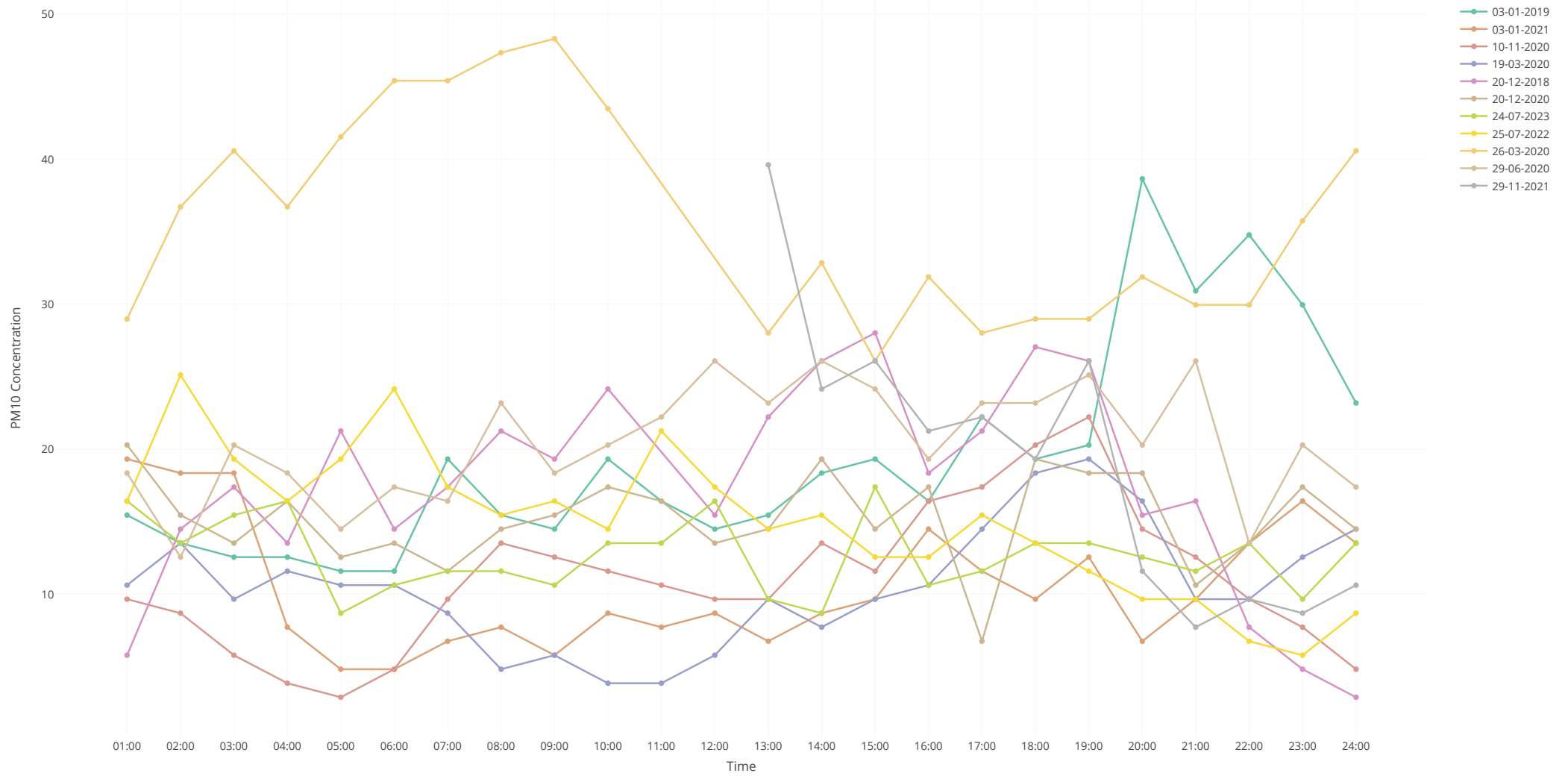
PM10 Levels by Date
